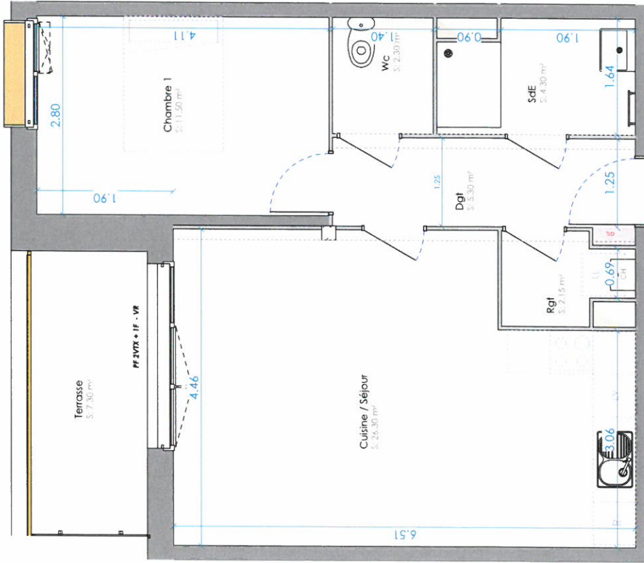
PLAN R+1
