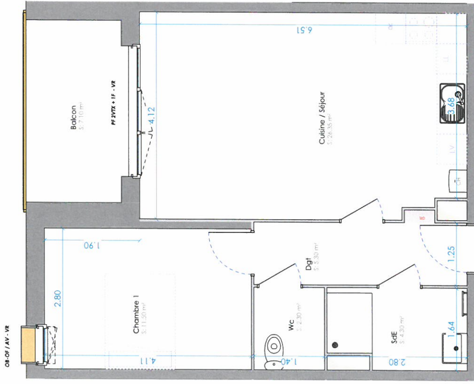
PLAN R+1
